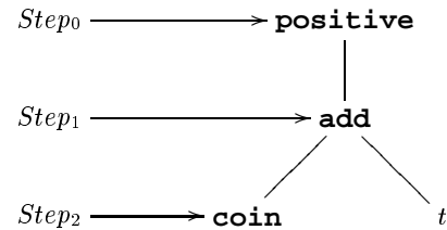
Figure 2: Snapshot of a computation of term positive(add(coin,t))
